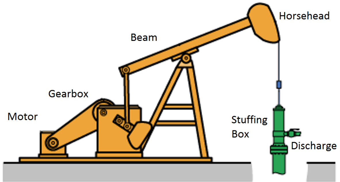
Figure 1: A schematic of a rod pump. The motor drives the gearbox, which causes the beam to tilt. This drives the horsehead up and down. This assembly assures that the rotating motion of the motor is converted into a linear up-down movement of the rod. The stuffing box contains the oil that is discharged through a valve on the top of the well.
