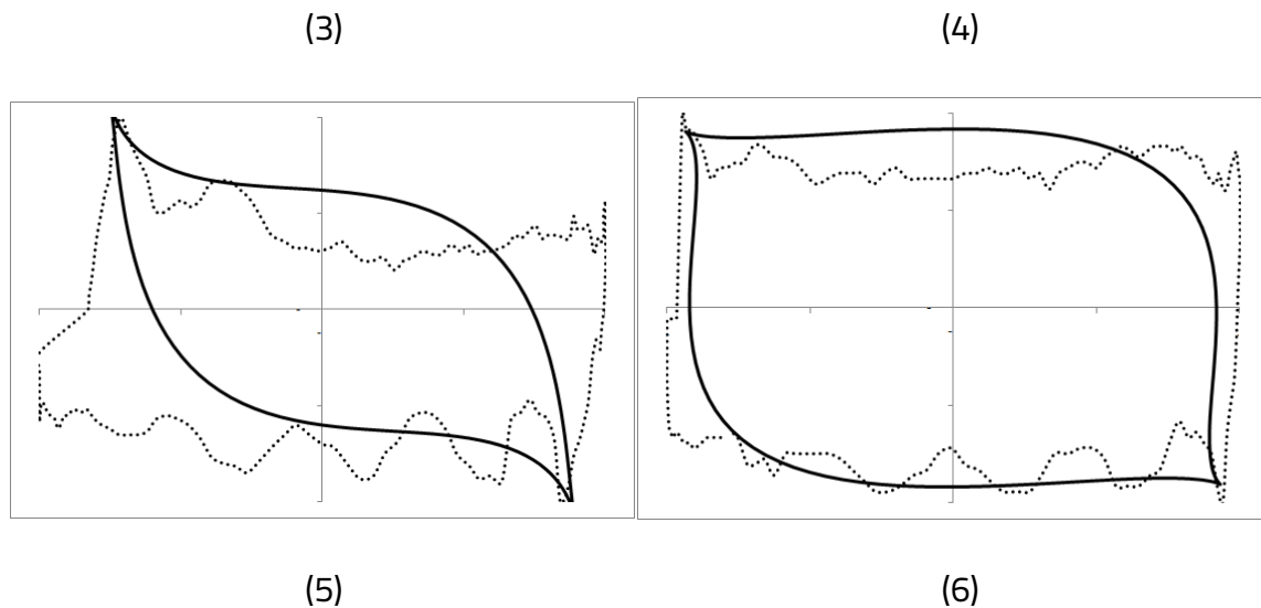
Figure 4: The modeling of a dynamometer card's evolution in time. Each card was measured 2000 pump cycles (about 8.3 hours) after the previous image. Images (1) and (2) at the top are historical data providing the model with the initial data. Using this, the model predicts images (3) to (5) and indicates that at image (5) we have a problem requiring attention. The maintenance measure is performed and we observe, see image (6), the establishment of operations as they should be.
