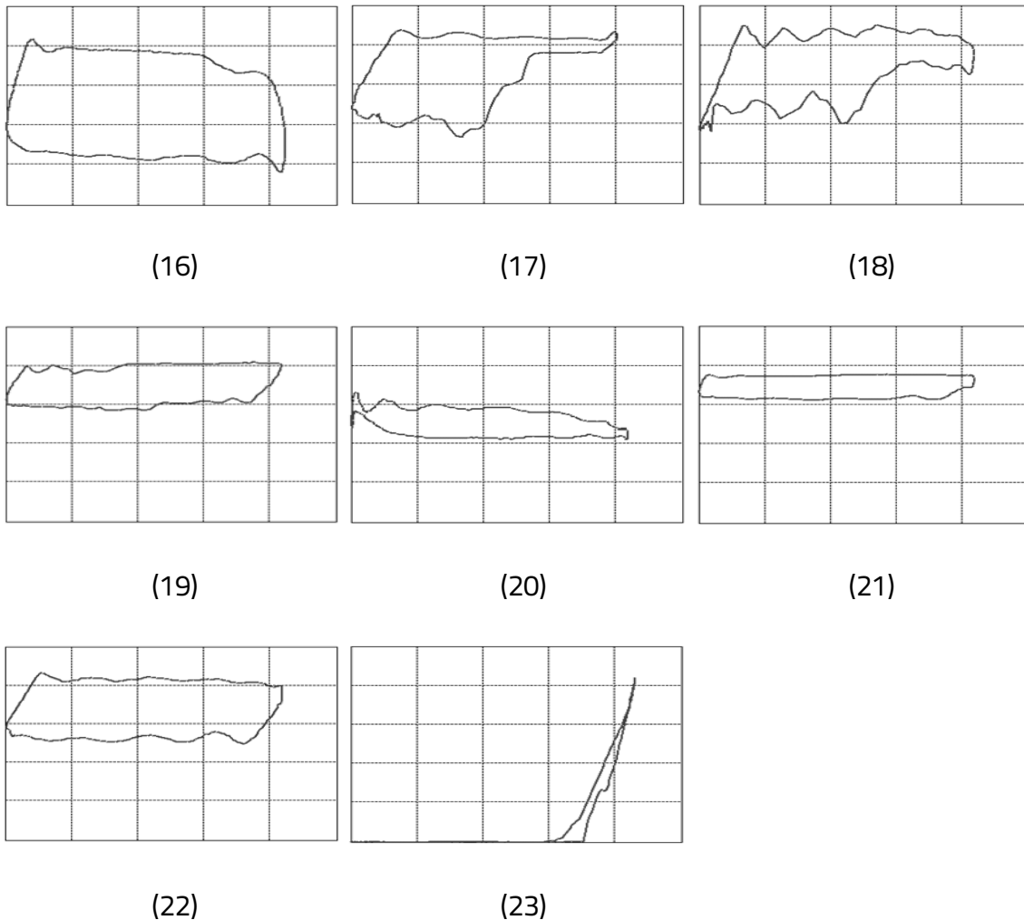
Figure 3: The various cases of dynamometer cards. See text below (points 1-23) for an explanation.
