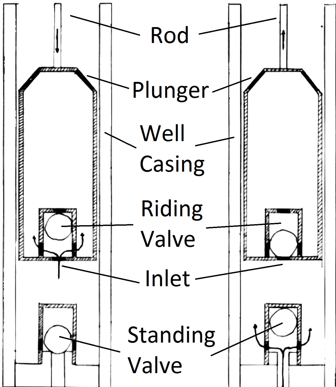
Figure 2: A schematic of the well bottom. The rod drives the plunger down into the well guided by the well casing. The bottom of the plunger has a so-called riding valve to take in the oil through the inlets. The bottom of the well is closed off to the reservoir with a so-called standing valve that opens once the plunger is at the bottom.
